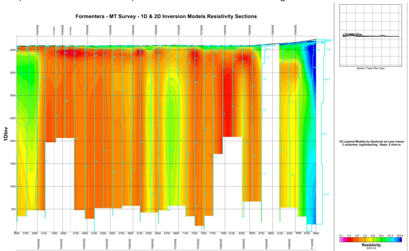
Figure 3. The above one dimension (1D) survey of line 1300 shows vertical lines of data and resistivity point values. The resistivity point values under 2.5 ohm-m show highly conductive areas that possibly contain lithium bearing aquifers. The orange is 0.9 ohm-m and the red 0.3 ohm-m. The non-conductive areas are in green and blue. The blank area on the east side is the road which for practical reasons could not be surveyed over.
