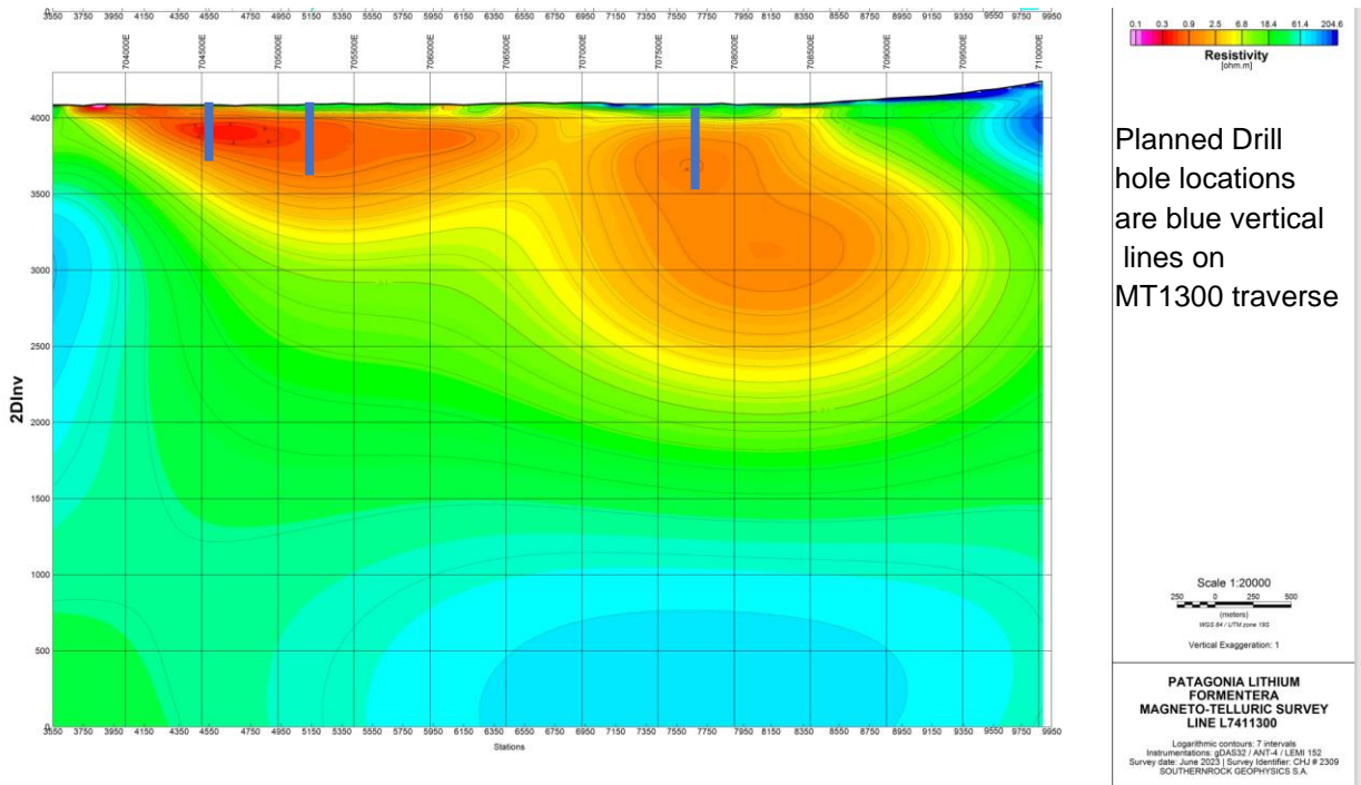
Figure 4. The 2D of line 1300 shows an elevation view with 750m thickness of a elliptical shaped aquifer with a resistivity below 0.9ohm-m and a large area adjacent to it with values less than 2.5 ohm-m. The blue lines show the proposed drill pattern. Three drill holes are planned on this line for a total of 1,000m.
