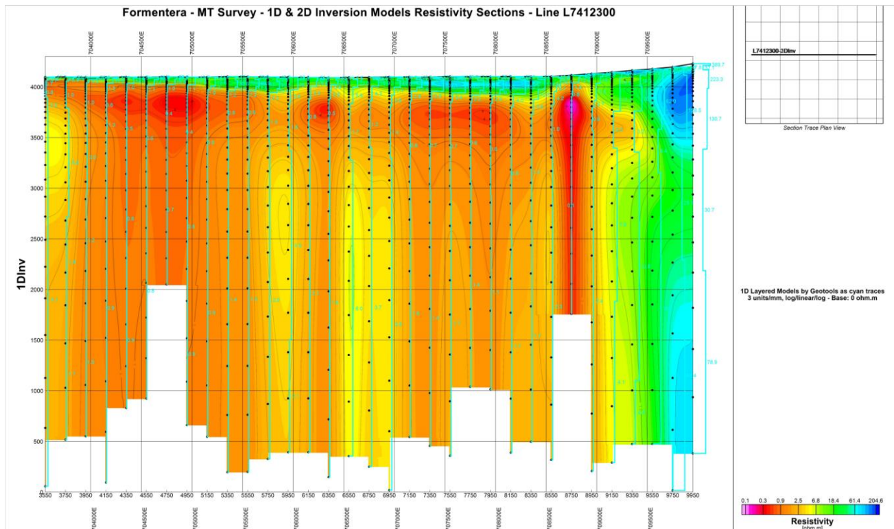
Figure 5. Line 2300 1D inversion shows an extremely low resistivity unit of 0.1ohm-m to the east (area in pink and red) and several areas between 3500m and 4000m in red that shows possibly a 300-400m thick aquifer.
