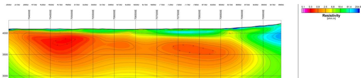
Figure 1. Low resistivity areas on line 2300 show very strong prospectivity and ideal drill targets.
