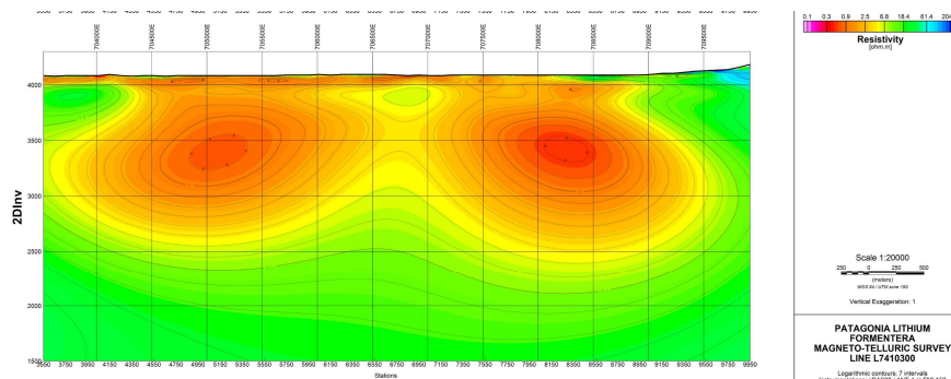
Figure 4. 2D inversion shows a large low resistivity area down to 2,500m ABSL (1,500m thickness) with a resistivity less than 2.5 Ohm-m.
