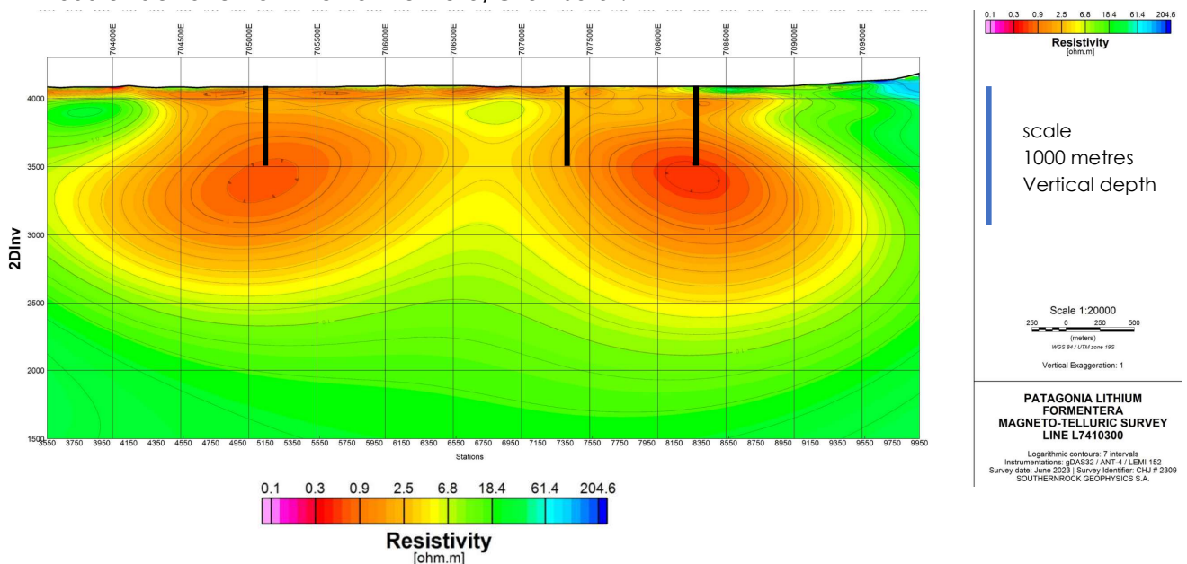
Figure 1. Low resistivity areas at 0.5-0.9 Ohm-m on line 0300 show very strong prospectivity and ideal drill targets.
