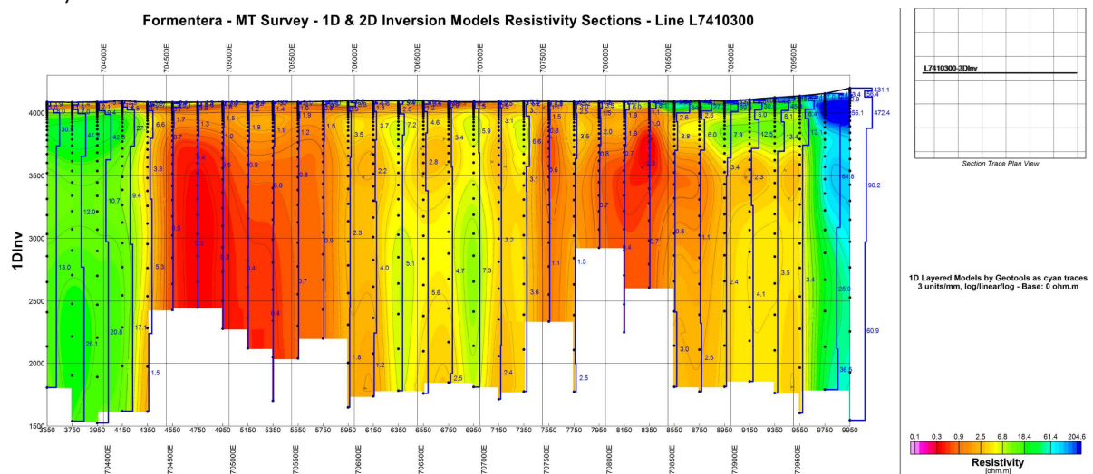
Figure 3. The above one dimension (1D) survey of line 0300 shows vertical lines of data and resistivity point values. The resistivity point values under 2.5 ohm-m show highly conductive areas (orange and red) that are very prospective for lithium bearing aquifers. The orange is 0.9 ohm-m and the red 0.3 ohm-m. The less conductive areas are in green and blue. The blank area on the east side is the road which for practical reasons could not be surveyed.
